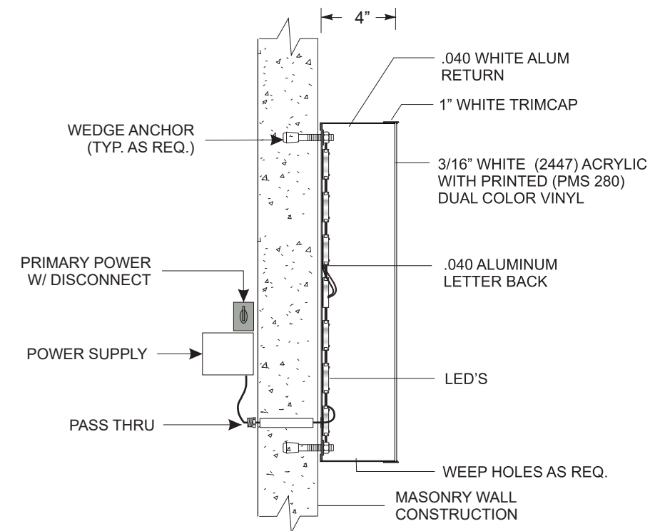
AA MC MOUNTING ON MASONRY CONSTRUCTION N.T.S.
