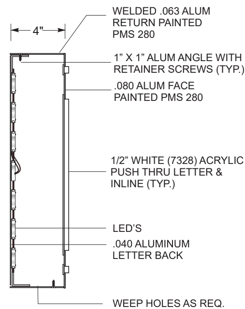
1-1 SECTION DETAIL AT CHANNEL LETTERS N.T.S.
