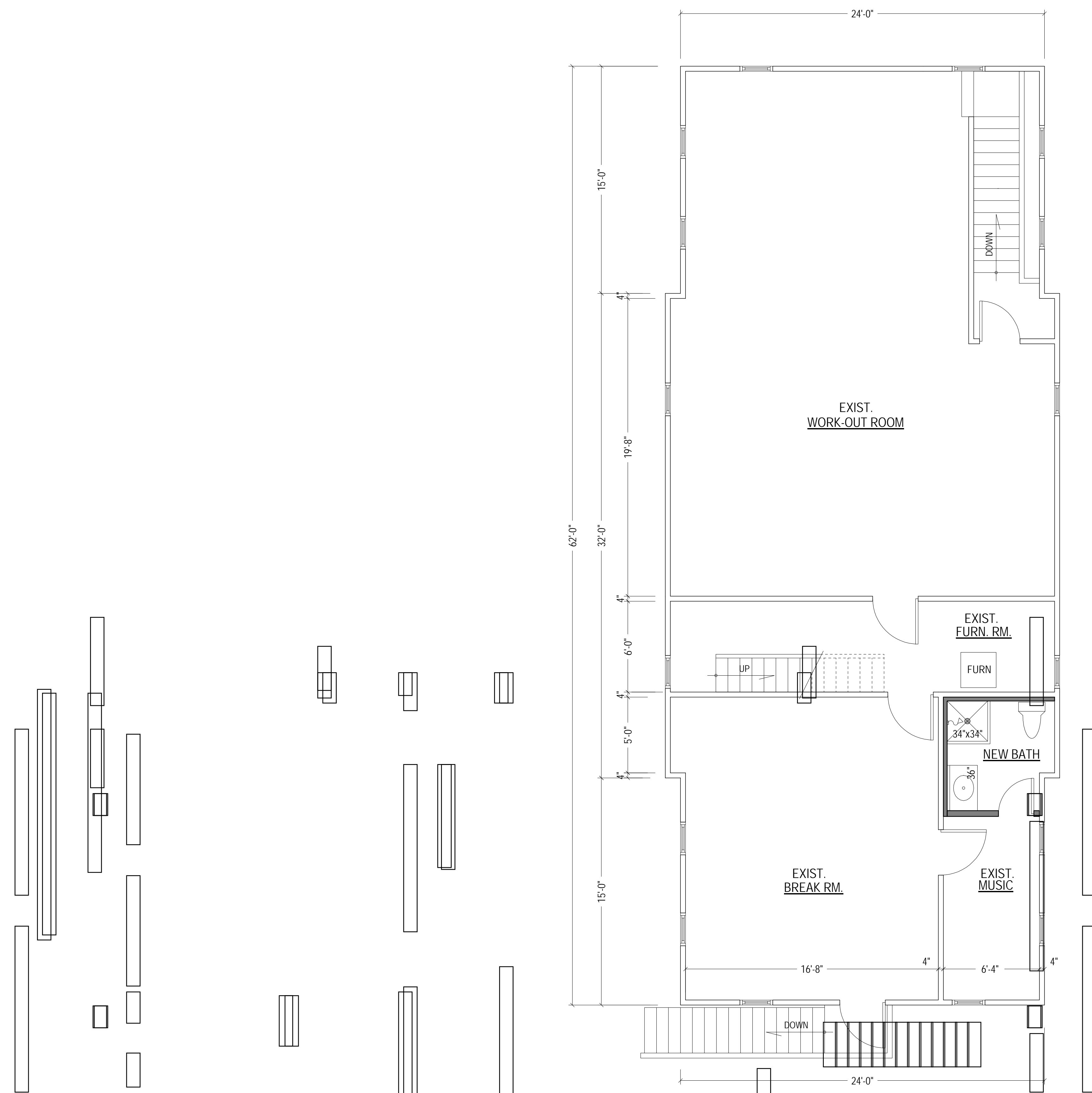
BARN - SECOND FLOOR SCALE: 1/4" = 1'-0"
